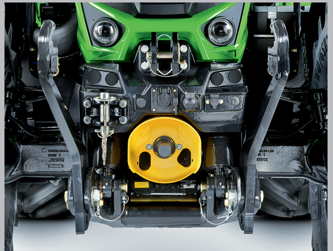
New front lift position control for more work capacity (only TTV models).
