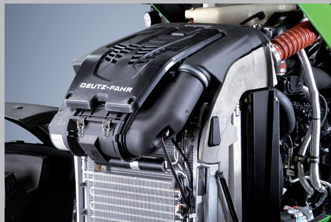
PowerCore technology air filter: 20% higher air flow capacity than comparable standard filters.
